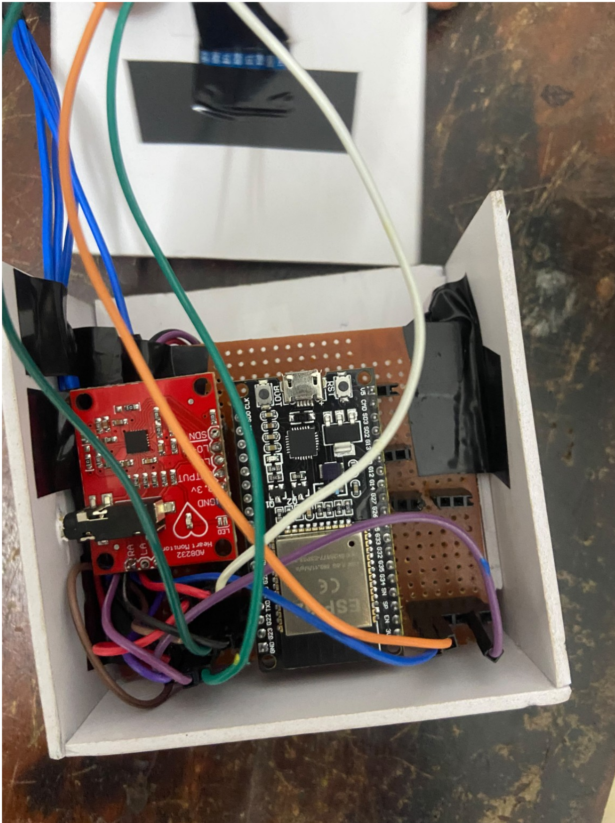
Figure 3: ESP32 and Sensor Hardware Prototype
